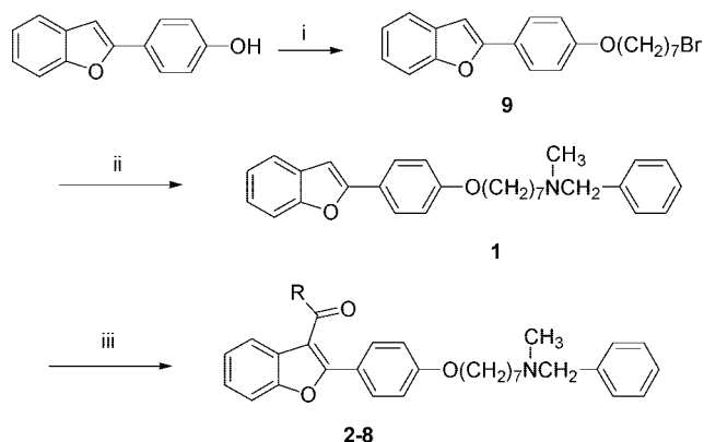
Scheme 1. Synthesis of the Studied Compounds a
